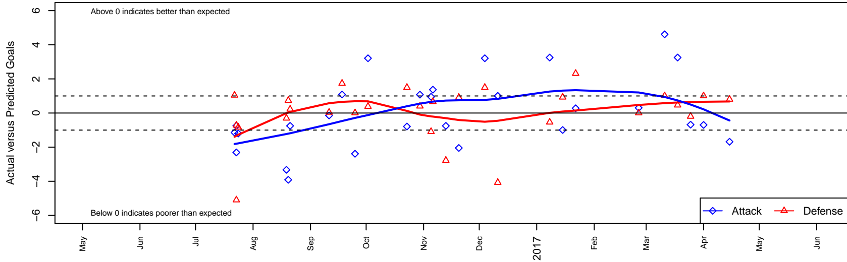
Newport FC Barca B02 Dots are actual minus expected GF (blue circles) and GA (red triangles). Blue line is smoothed change in attack strength. Red is smoothed change in defense strength.
